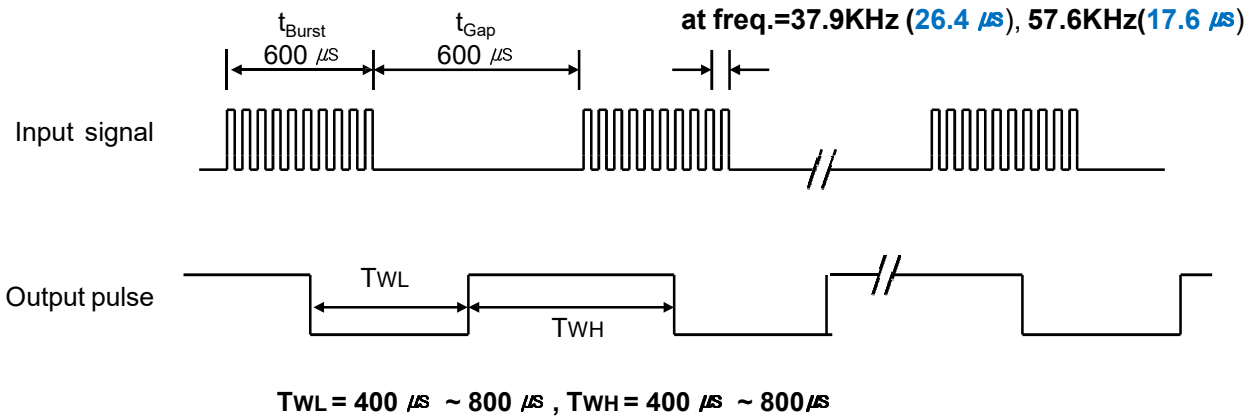
[ Fig.1 ] Output Waveform
